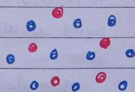
High Entropy
